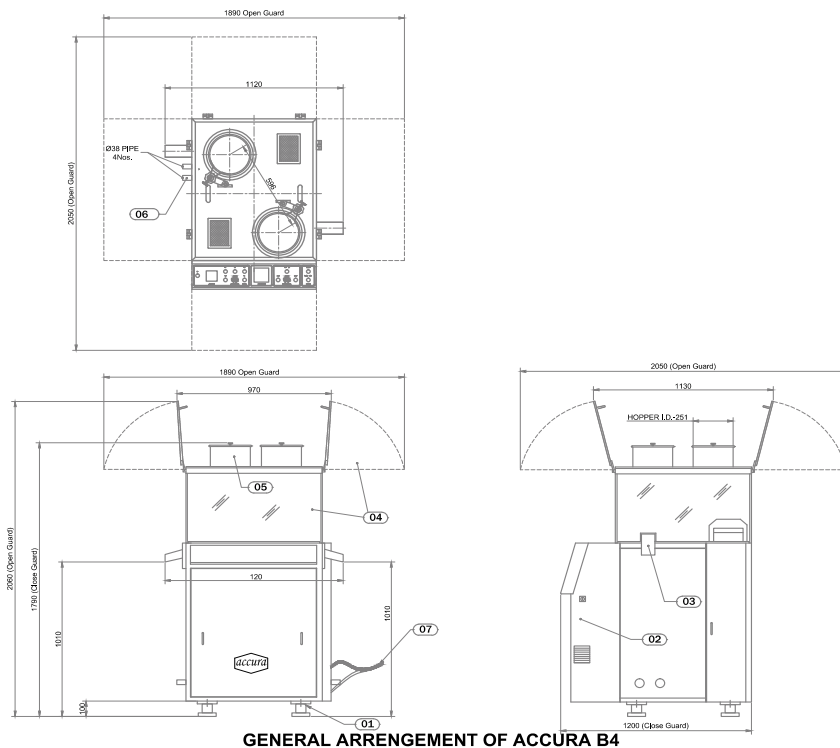
GENERAL ARRANGEMENT OF ACCURA B4
